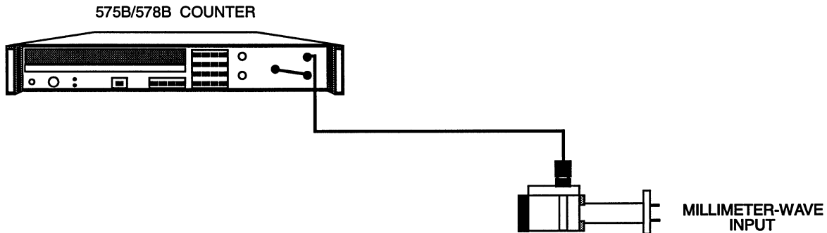
Figure 3-8. Equipment Setup for Band 4 Operation (Option 06)
